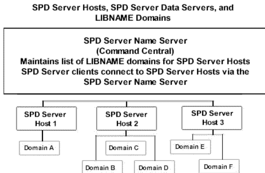
Figure 3.1 SPD Server Hosts, SPD Server Name Servers, and LIBNAME Domains
